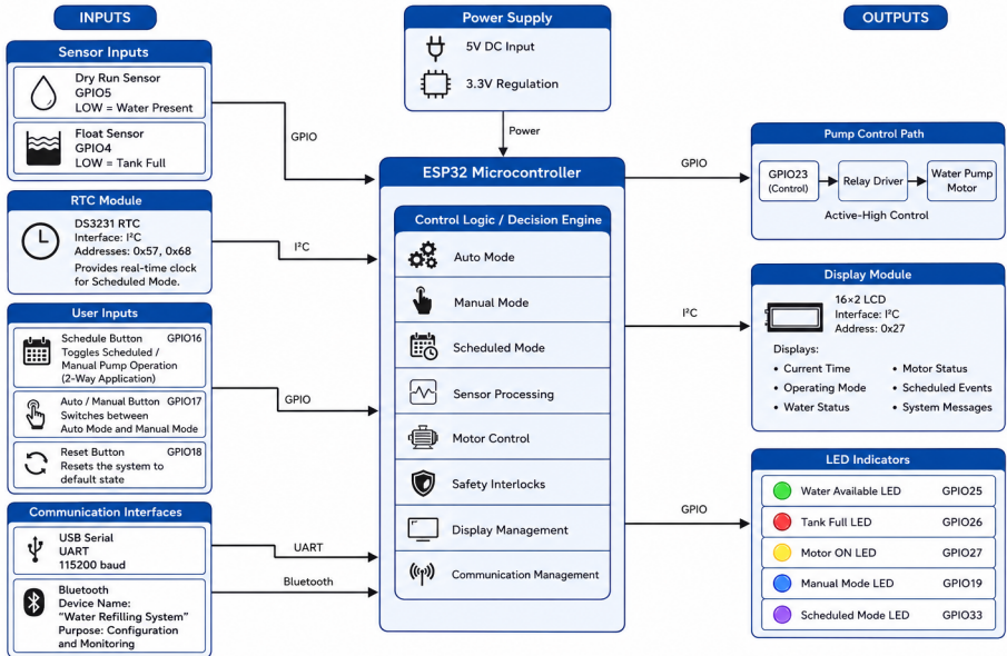
ESP32-BASED SMART WATER REFILLING SYSTEM
